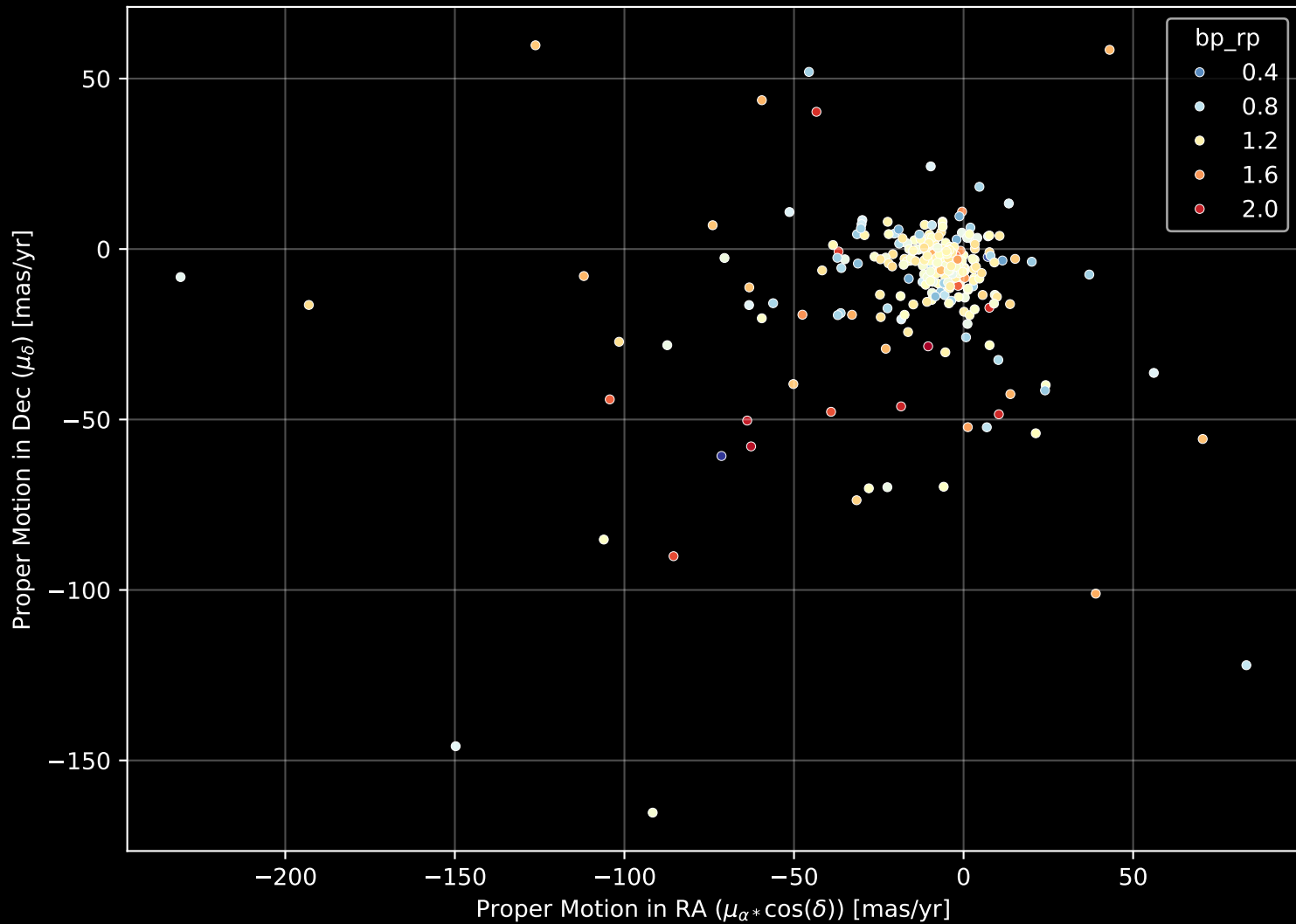
APOGEE DR17 Field: [N5634SGR2] Proper Motion Diagram (n= 304)
