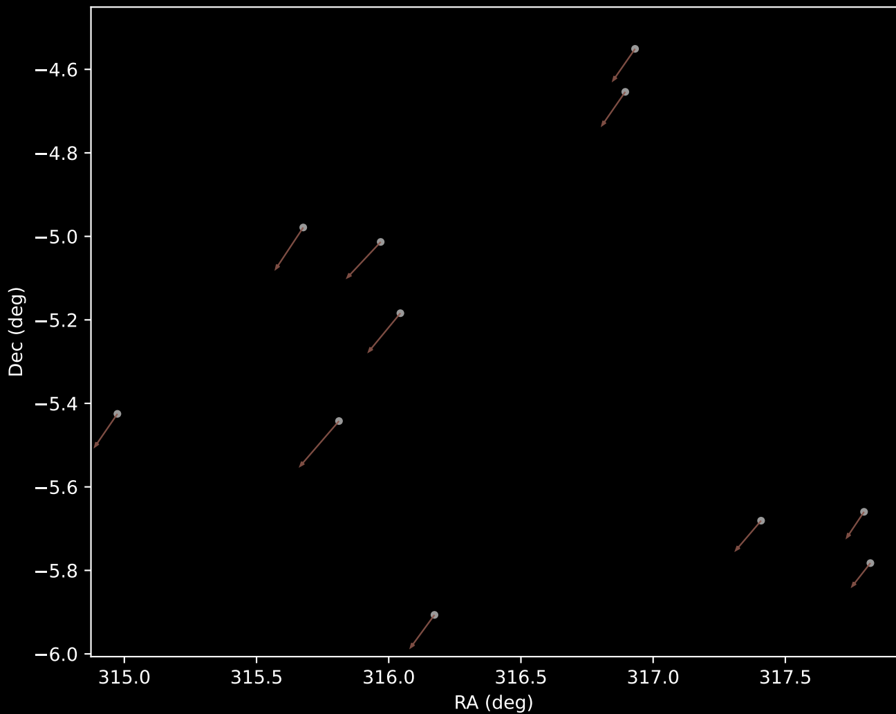
APOGEE DR17 Cluster 10 Proper Motion Vectors (n=11)
