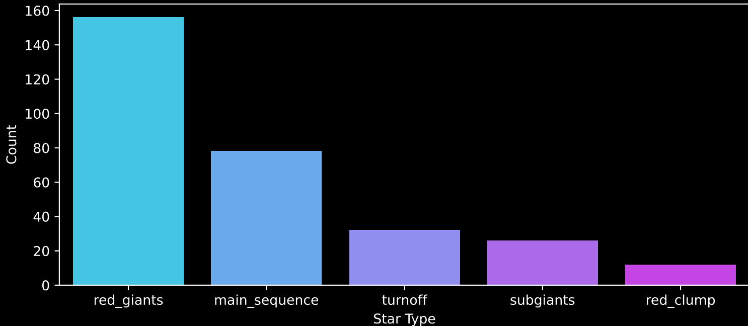
APOGEE DR17 Field: [N5634SGR2] Count plot of Star Type
