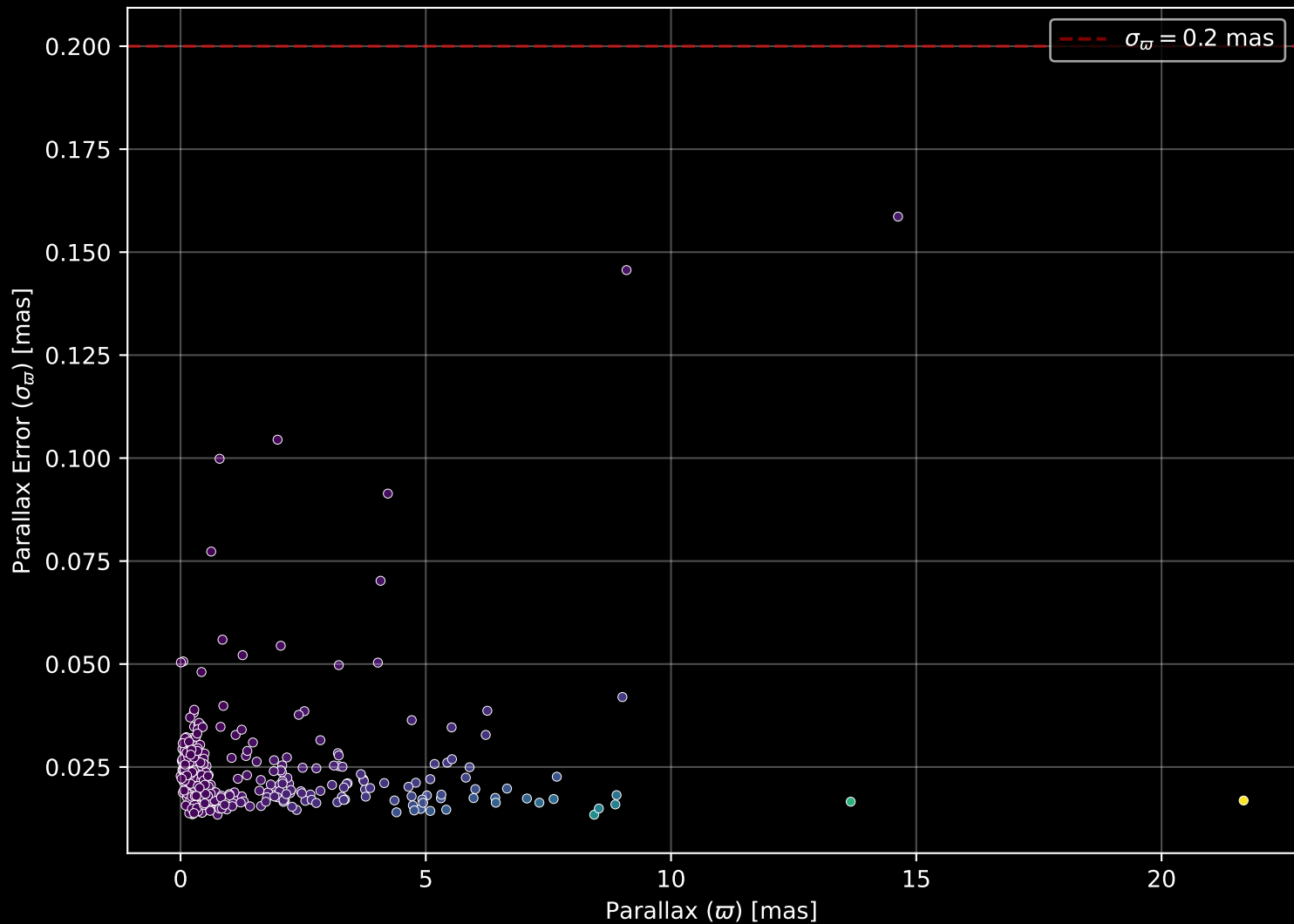
APOGEE DR17 Field: [N5634SGR2] Parallax Quality (n= 304)
