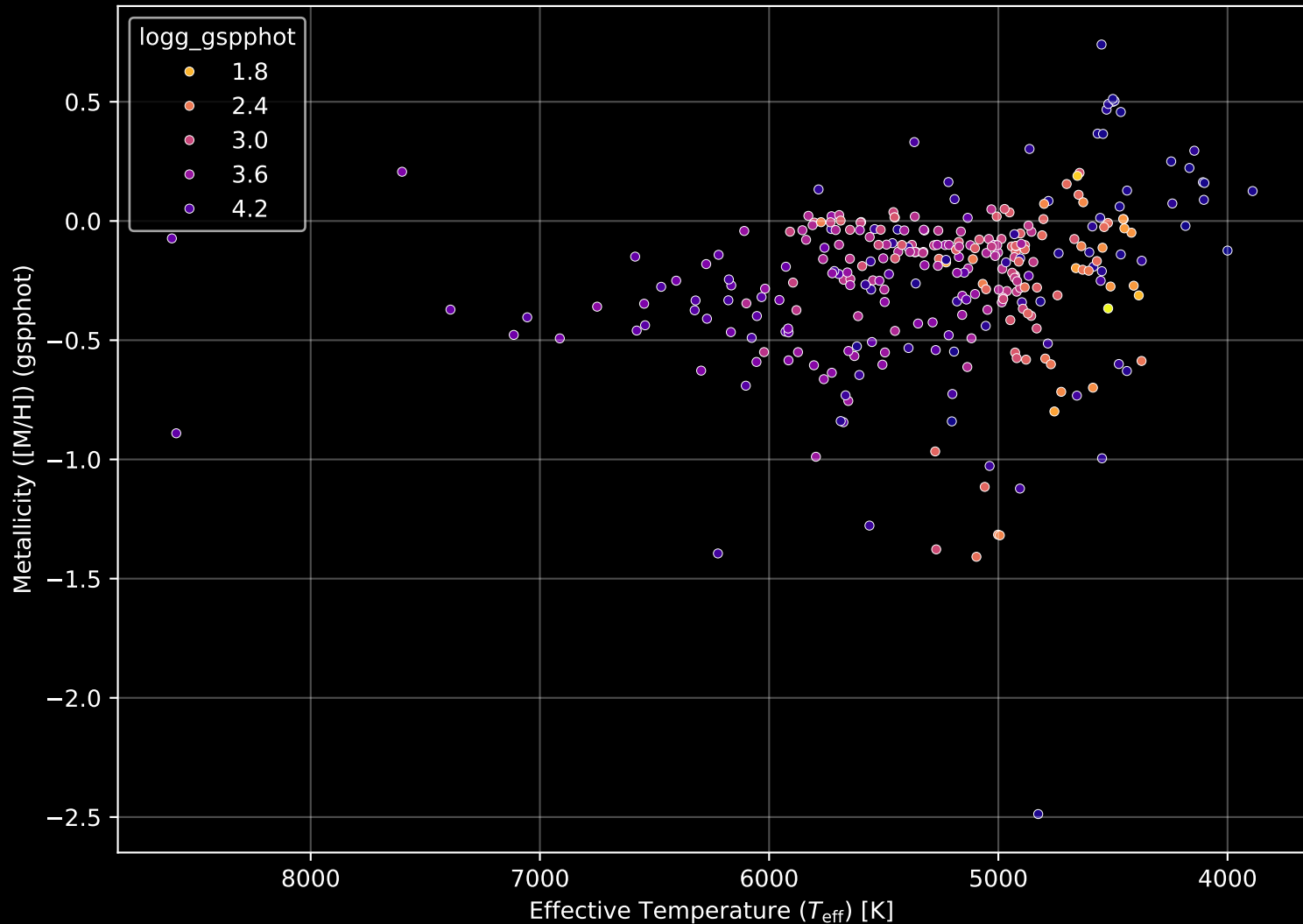
APOGEE DR17 Field: [N5634SGR2] Stellar Population Parameters (n= 304)
