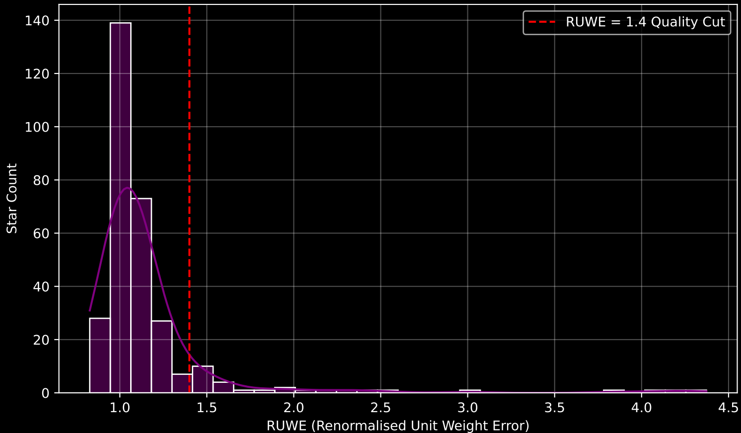
GAPOGEE DR17 Field [N5634SGR2] RUWE Distribution (n= 302)
