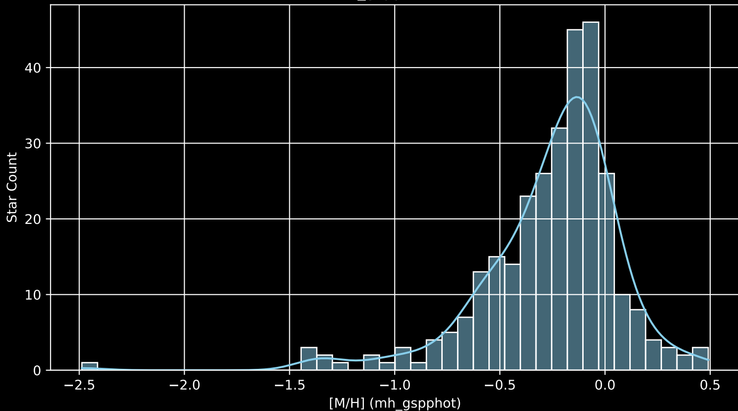
APOGEE DR17 Field: [N5634SGR2 [M/H] (mh_gspphot) (n= 300)
